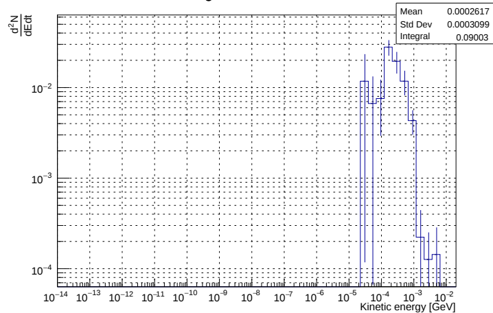
NEUTRON ♦ reg 3 → 2 ♦ Time: 0.01 to 1000 s
