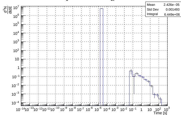
NEUTRON ♦ reg 3 → 2 ♦ Kinetic energy: 1\text{e-}14 to 0.02 \text{ GeV}
