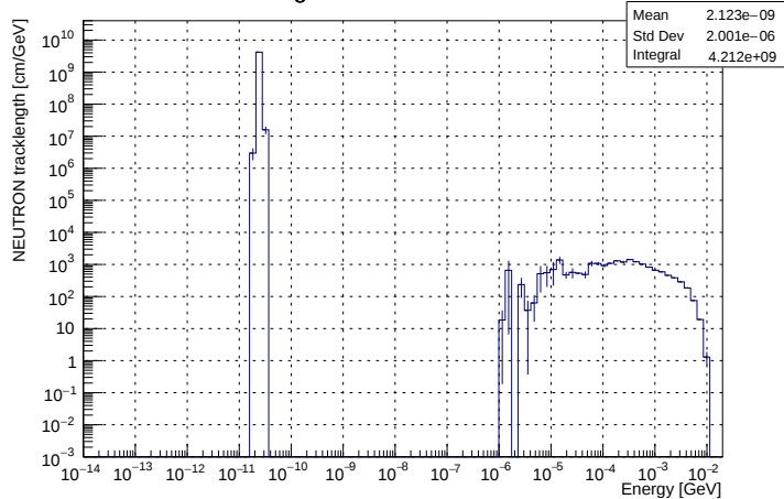
NEUTRON ♦ reg 3 ♦ 1 \text{ cm}^3 ♦ 1\text{e-}14 < E < 0.02 \text{ GeV}
