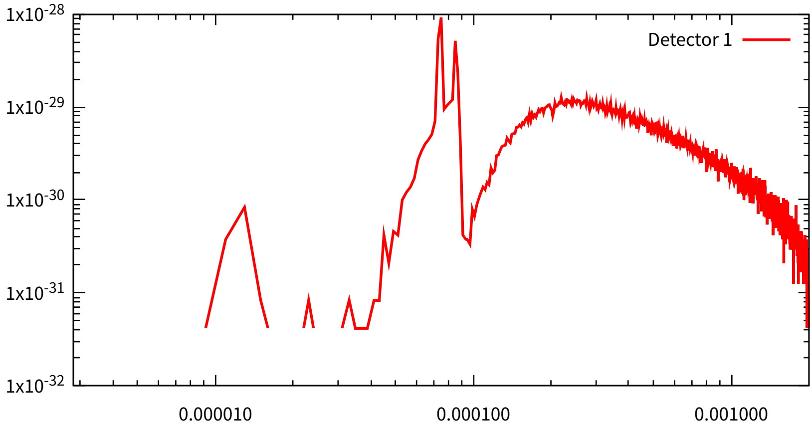
USR-1D electron brems 31
