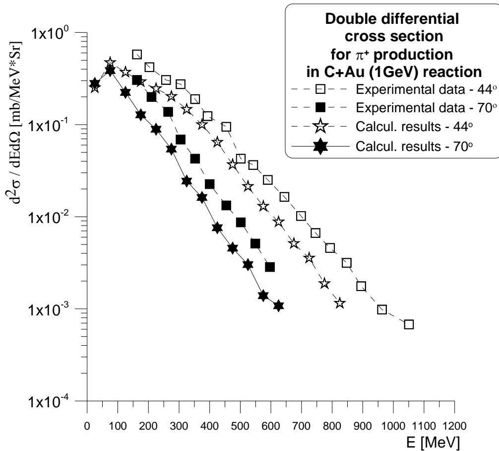
Fig2. Double differential cross section for \pi^+ in C+Au(1GeV) reaction. Experimental data are from [1]. Calculation results are from FLUKA code.
