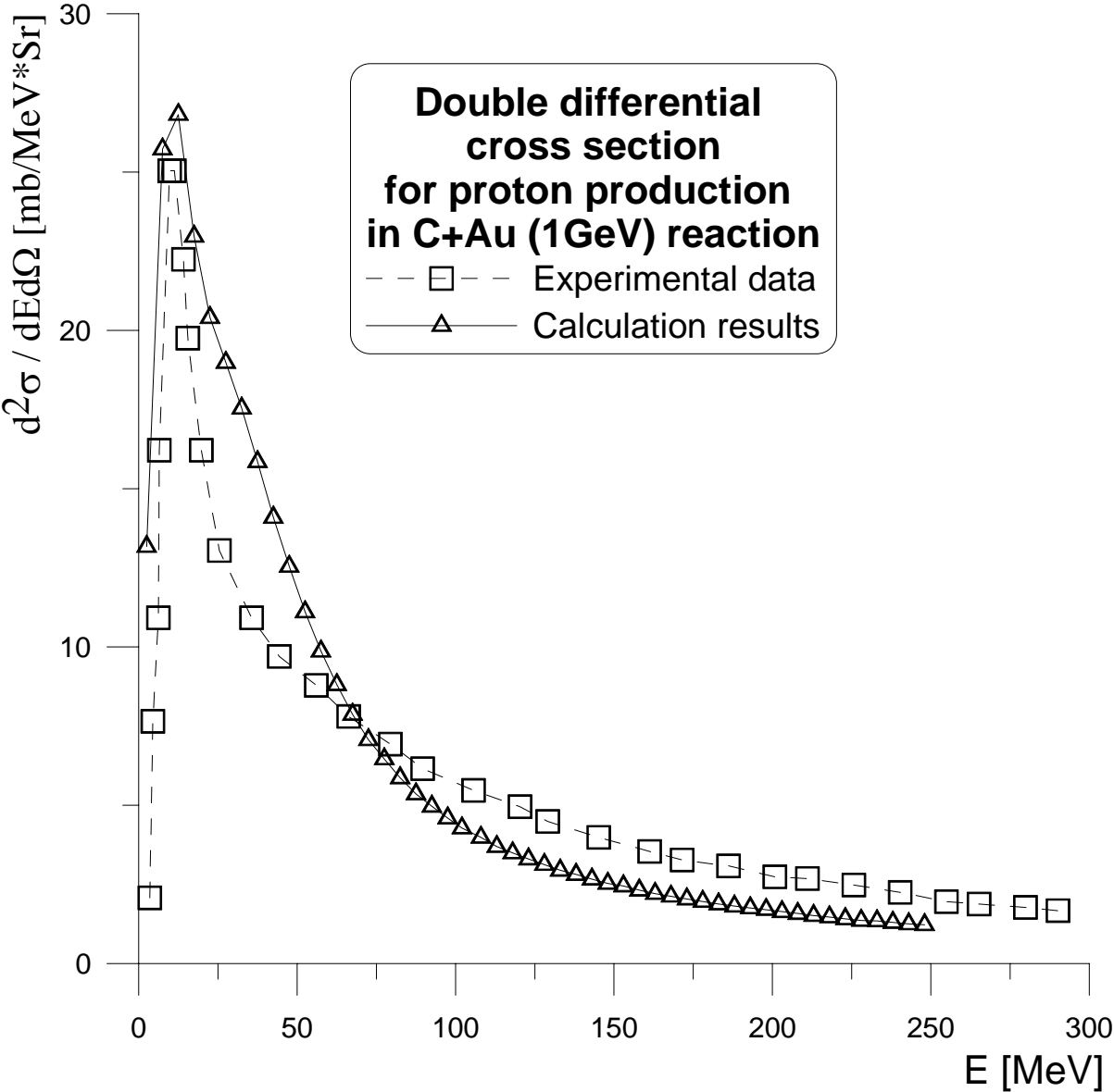
Fig1. Double differential cross section for protons in C+Au(1GeV) reaction. Experimental data are from [1]. Calculation results are from FLUKA code.
