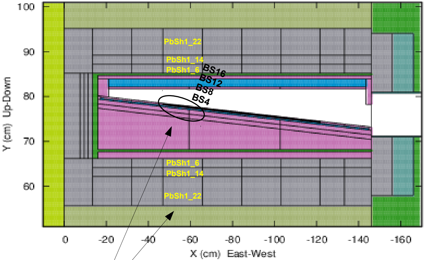
eLinac BD9: Geometry - Side View - BD (Z = 98.5 cm from the North Wall)
