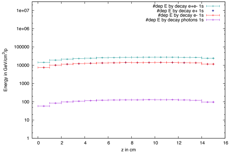
deposited Energy by decay products in 15 cm long YSO crystal after 1 s
